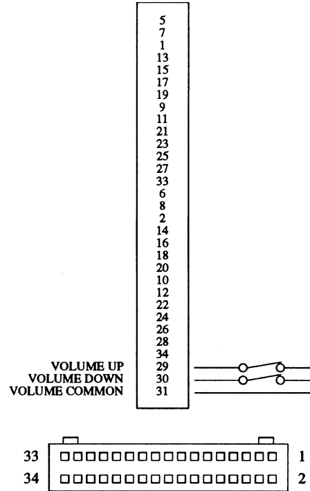
Harness Side
